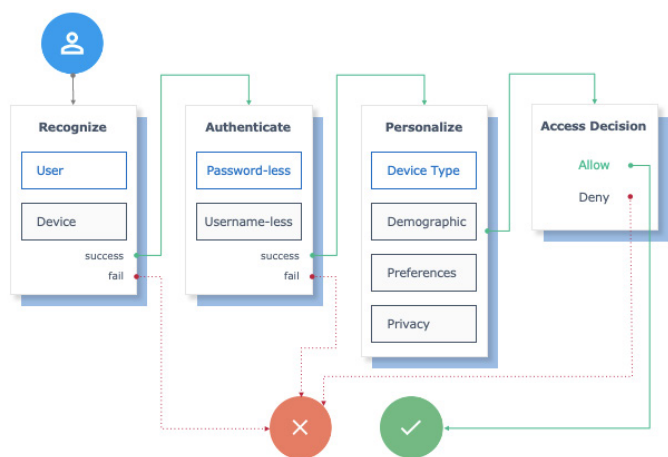
Figure 2: Designing Dynamic User Journeys with ForgeRock Intelligent Access
